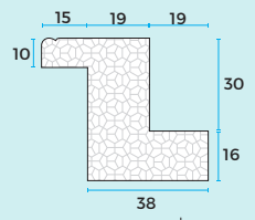
TEXAS Z FRAME P4013
