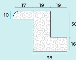
BULLNOSE Z FRAME P4033
