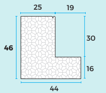
L FRAME P4001N
