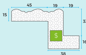
FANCY Z FRAME P4014
