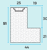
51mm L FRAME F/F P4008H
