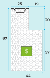
87mm L FRAME F/F P4008T
