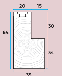
64mm L FRAME F/F 4008B
