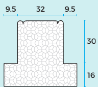
BEADED T POST P7032
