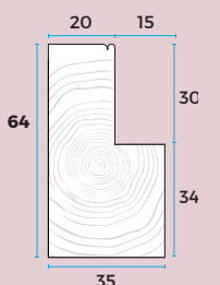
64mm L FRAME 4001B
