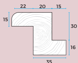
BULLNOSE Z FRAME 4003
