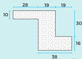
PLAIN Z FRAME P4073
