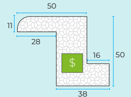
LARGE BULLNOSE Z FRAME P4014
