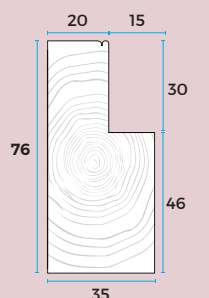
76mm L FRAME 4001C
