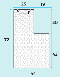
72mm L FRAME F/F P4008S
