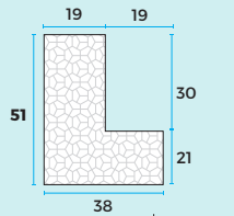
L FRAME P4007A
