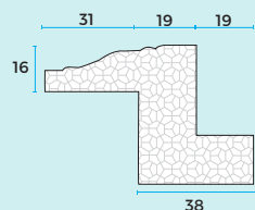
COLONIAL Z FRAME P4043
